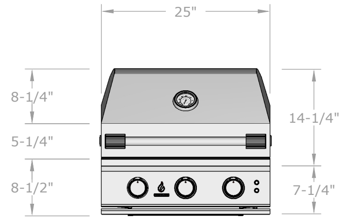
FRONT VIEW SCALE 1:14
