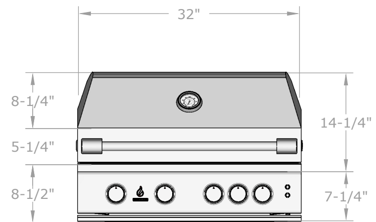
FRONT VIEW SCALE 1:14
