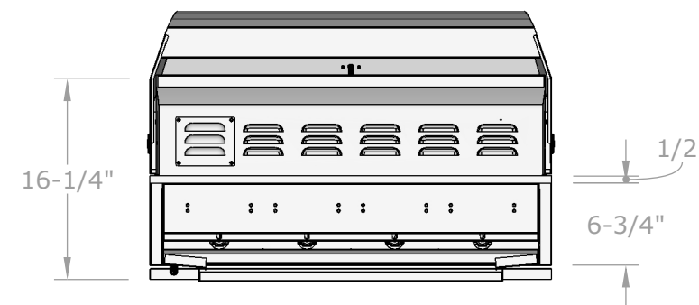
BACK VIEW SCALE 1:14
