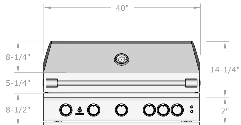
FRONT VIEW SCALE 1:14
